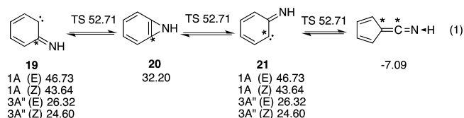
Scheme 2. The Cycloperambulatory Mechanism 12 (* = 13 C label)
