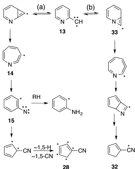
Scheme 8. The New Pathways of Ring Contraction of 2-Pyridylcarbene 13 (* = 13 C)
