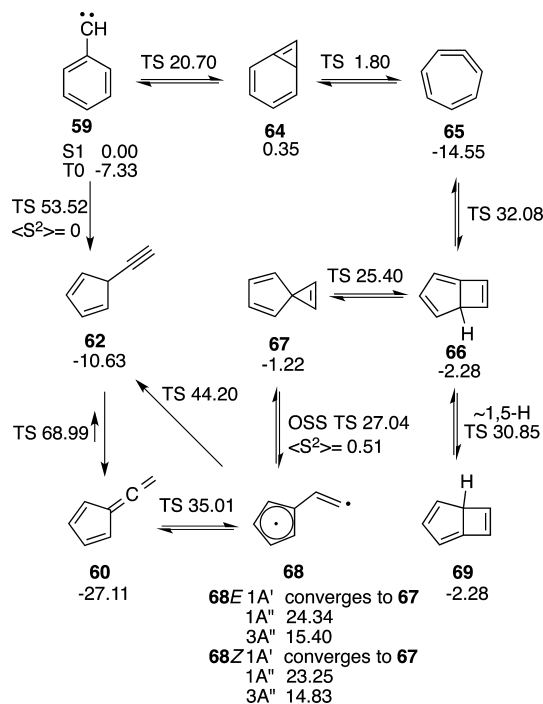
Scheme 12. Calculated Energies at the B3LYP/6-31G* + ZPVE Level Relative to Phenylcarbene S_1 (–270.115340 hartree) a
