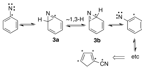
Scheme 2. The Cycloperambulatory Mechanism 12 (* = 13 C label)
