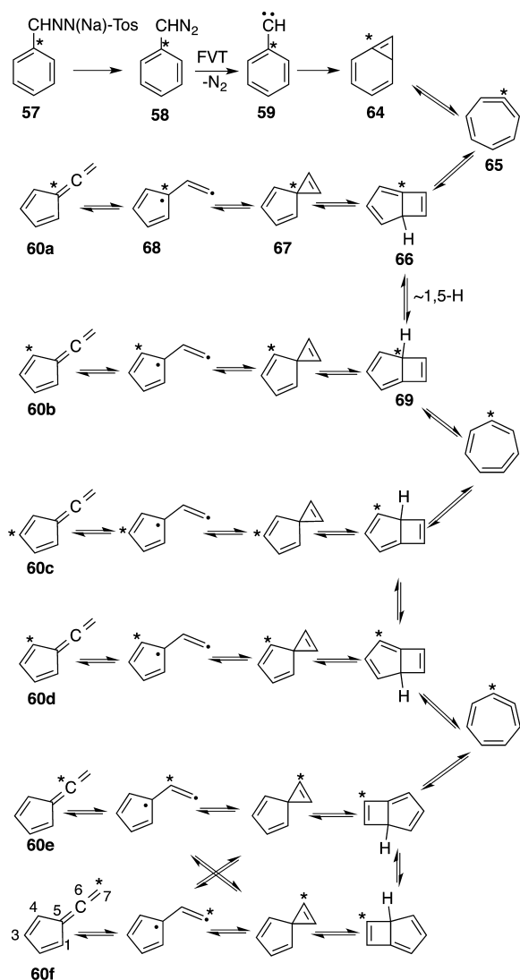
Scheme 11. Phenylcarbene–Fulvenallene Rearrangement, 60 atom-% ^{13}\text{C} in 57 (* = ^{13}\text{C} label)
