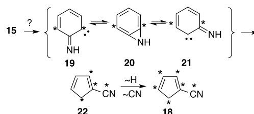
Scheme 5. Formation of 13 C-Cyanocyclopentadiene from 7a- 13 C-Isatin at 715 °C/0.15 mbar
