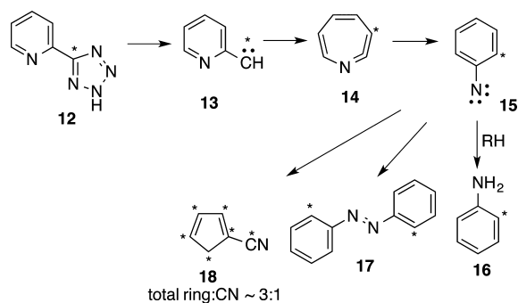
Scheme 3. Observed Products Derived from the 2-Pyridylcarbene–Phenylnitrene Rearrangement
