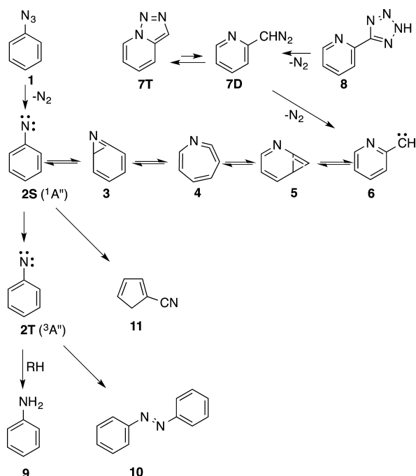
Scheme 1. Products of Thermolysis of Phenyl Azide 1 and 2-Diazomethylpyridine 7 and Interconversion of Phenylnitrene 2S and 2-Pyridylcarbene 6 a
