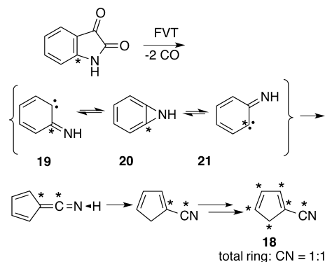
Scheme 5. Formation of 13 C-Cyanocyclopentadiene from 7a- 13 C-Isatin at 715 °C/0.15 mbar
