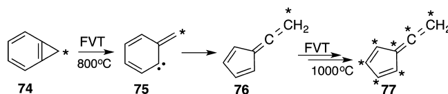
Scheme 14. FVT of Benzocyclopropene (* = 12 C, 13 C-depleted)
