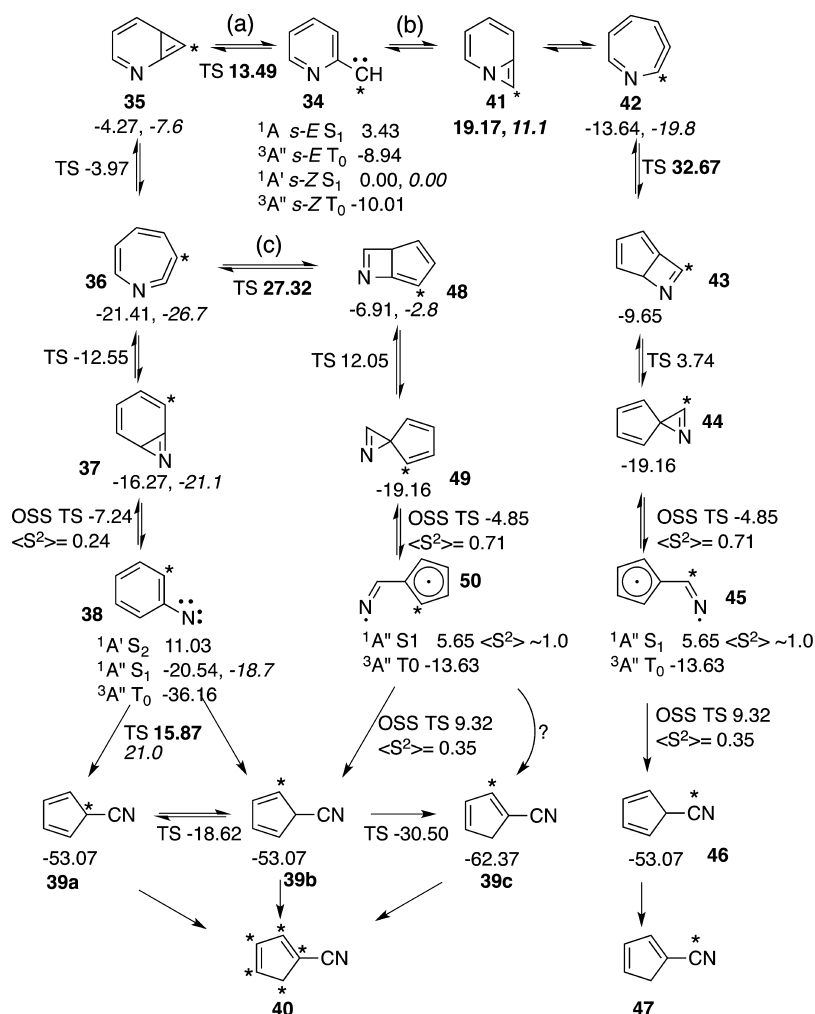
Scheme 9. Calculated Energies in kcal/mol Relative to s -Z-2-Pyridylcarbene 34S 1 (−286.158765 hartree) a
