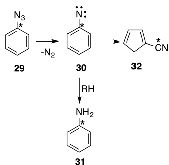
Scheme 7. Products of FVT of 1- 13 C-Phenyl Azide (* = 13 C)
