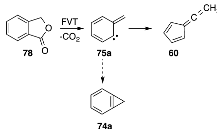
Scheme 15. Synthesis of Fulvenallene from Phthalide
