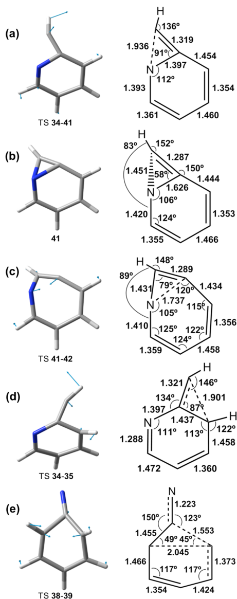
Figure 1. Structures of (a) TS34-41 (2-pyridylcarbene ring closure to N1), (b) azirine 41, (c) TS41-42 (ring expansion of 41), (d) TS34-35 (2-pyridylcarbene ring closure to C3), (e) TS38-39 (phenylnitrene-cyanocyclopentadiene) with displacement vectors, bond lengths (Å), and bond angles at the CASSCF(8,8)/6-31G* level. Structures at the B3LYP/6-31G* level are shown in the Supporting Information, Figure S8.
